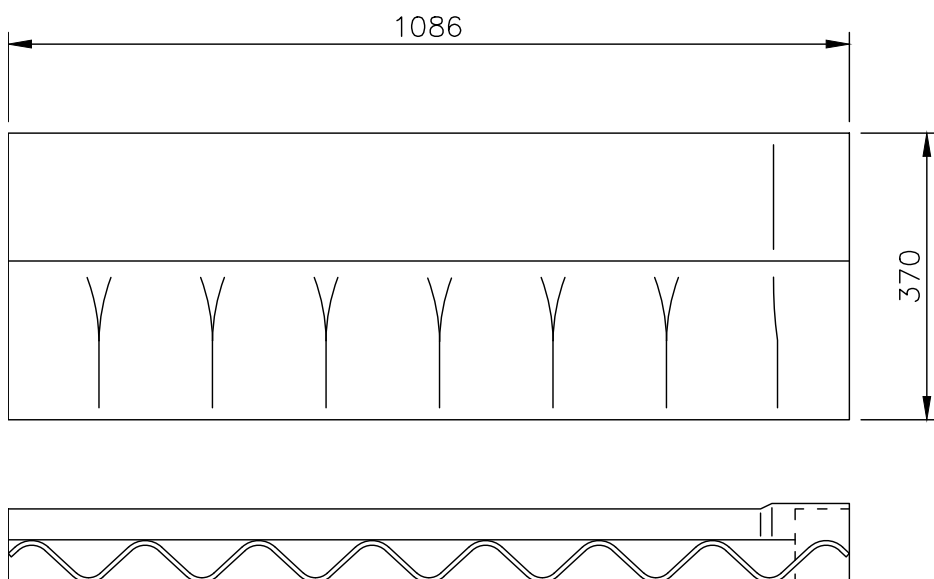
CEMBRIT LIMITED CEMSIX TWO-PIECE CLOSE FITTING RIDGE INNER (RIGHT) WING: 370mm NET COVER: 1016mm Drg. No.320
